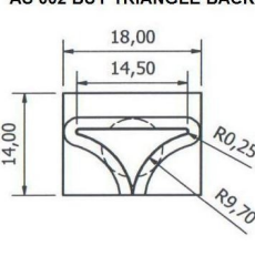
AS 002 BUT TRIANGLE BACK
